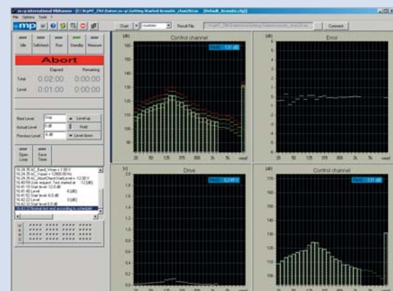
Spacecraft is tested in an acoustic reverberation chamber to represent the environments during lift-off
