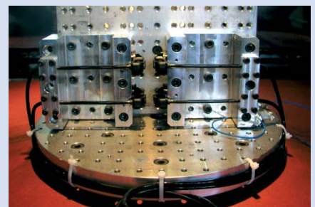
Vibration control on automotive connectors, Hirschmann Automotive GmbH, Rankweil/Austria
